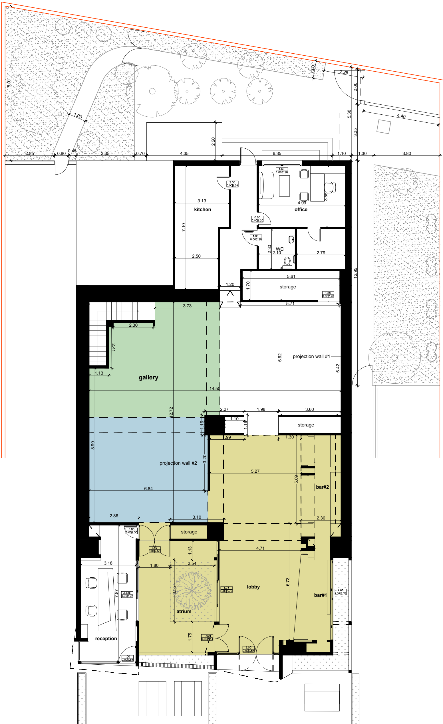
FLOORPLAN
